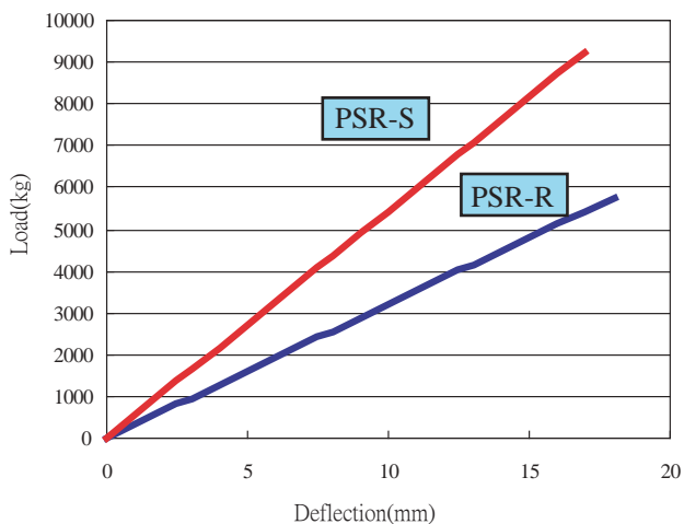
Load/Deflection Curves
