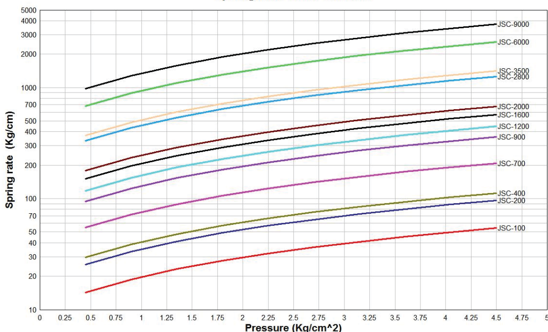
Spring rate of air mounts
